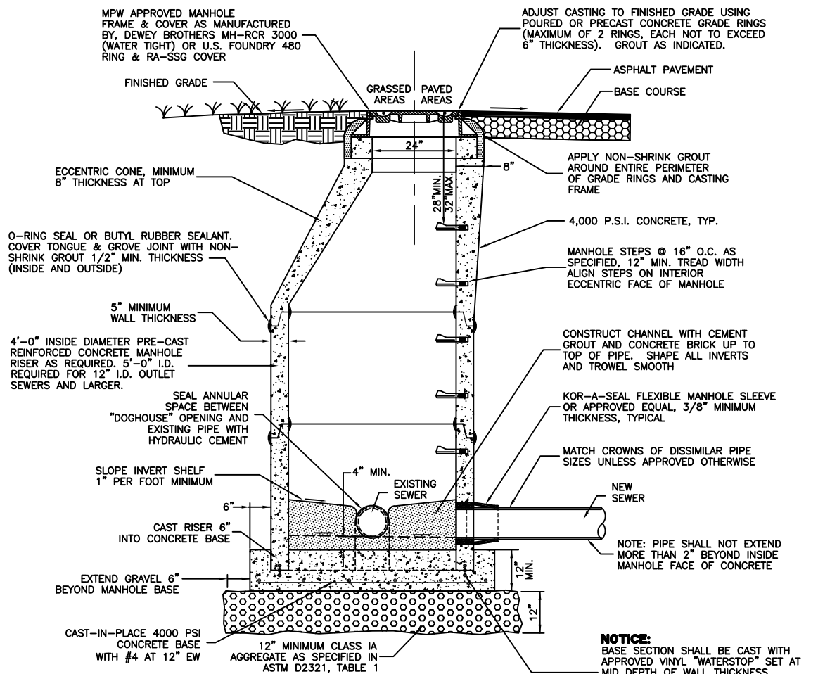
NEW MANHOLE OVER EXISTING SEWER SECTION NOT TO SCALE
