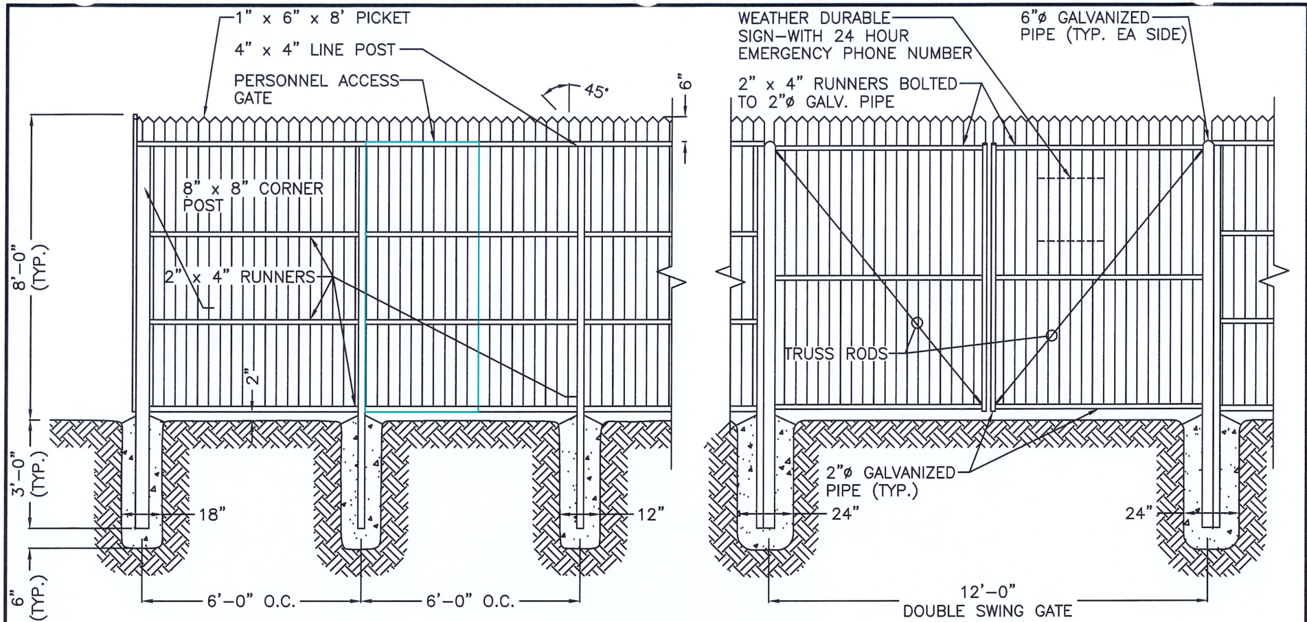
FRONT (INSIDE) VIEW
