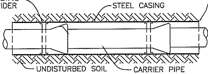
TYPICAL SECTION
